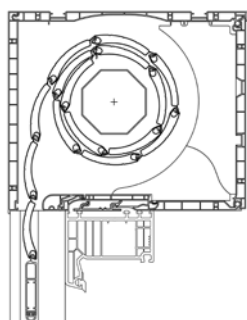
ROLLLADEN – REVISION INNEN
